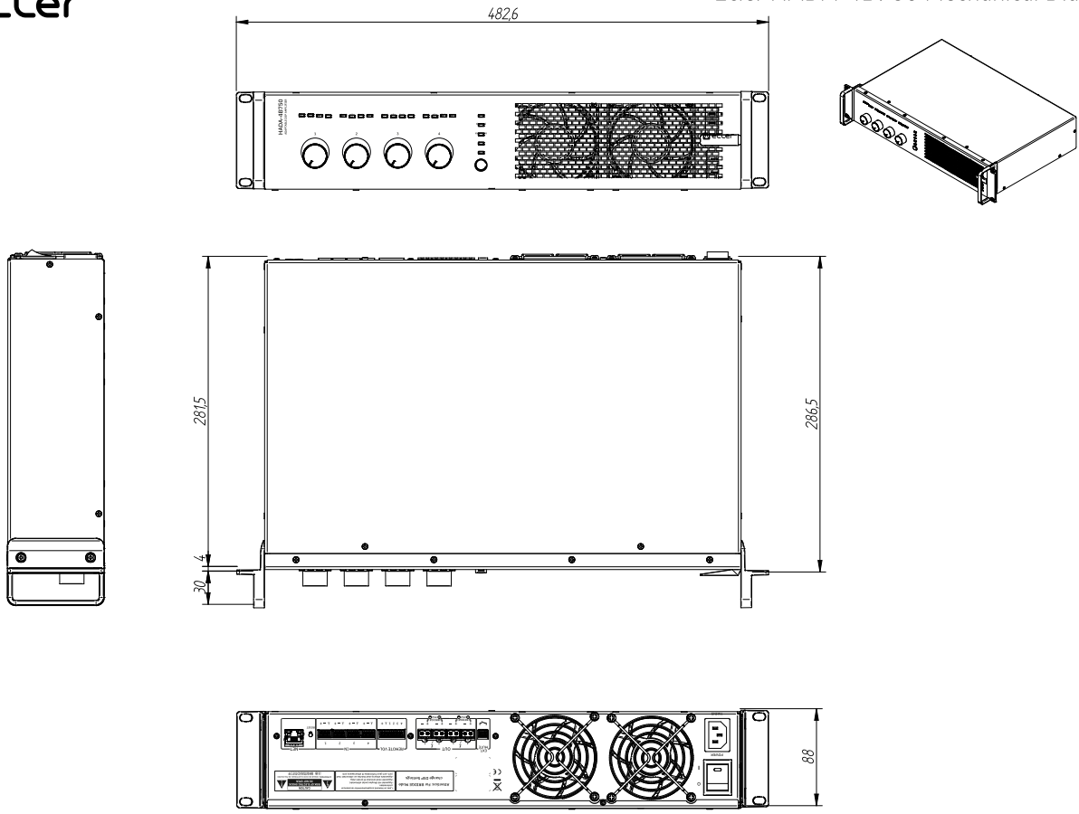
Ecler HADA-4B750 Mechanical Diagram
